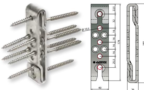
Standard screwing without clip lock.
