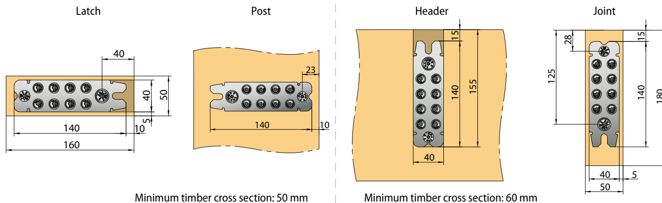
Minimum timber cross section: 50 mm
