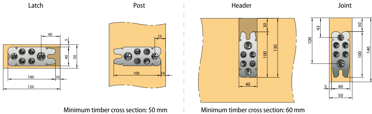
Minimum timber cross section: 50 mm
