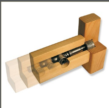
... of table legs with easy-con ®
